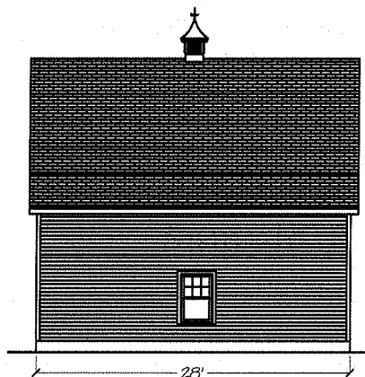
Left Elevation
